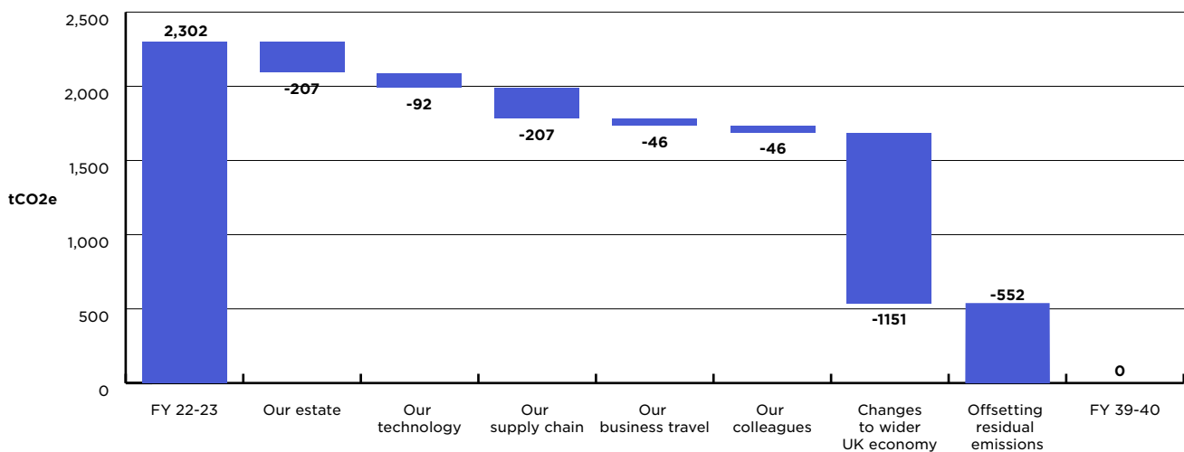
Figure 6 - Contribution of priority areas to journey to net zero for all scopes
