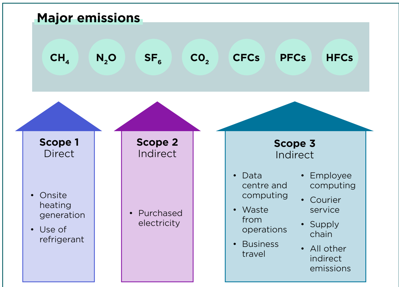
Figure 1 - The NMC's greenhouse gas emissions are reported within three scopes
