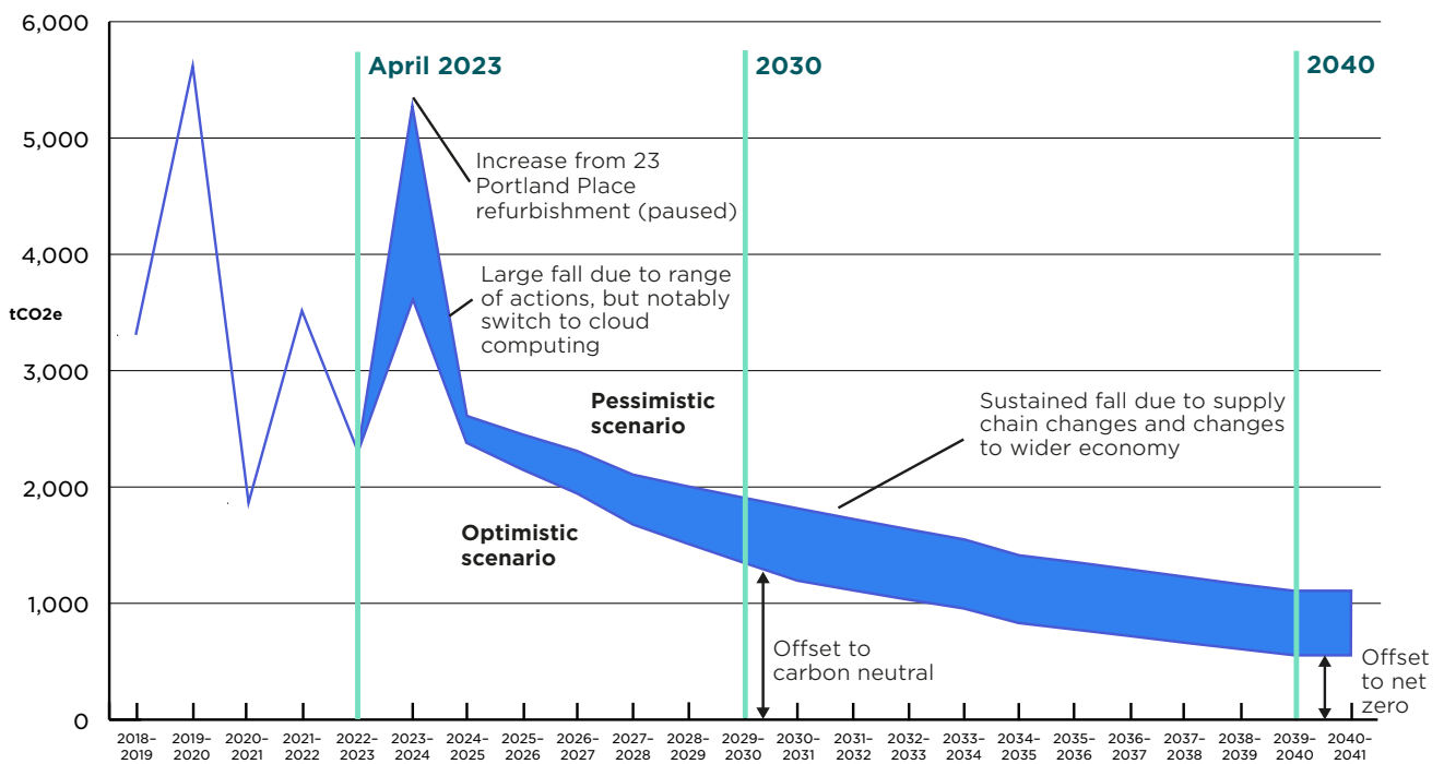
Figure 5 - Projected trajectory to net zero for all scopes
